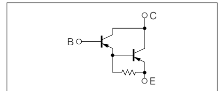
Internal Connection
